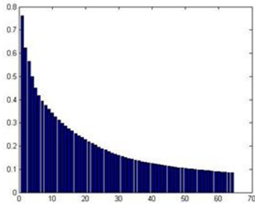
Figure 3 Error rate of training set for 65 iterations
