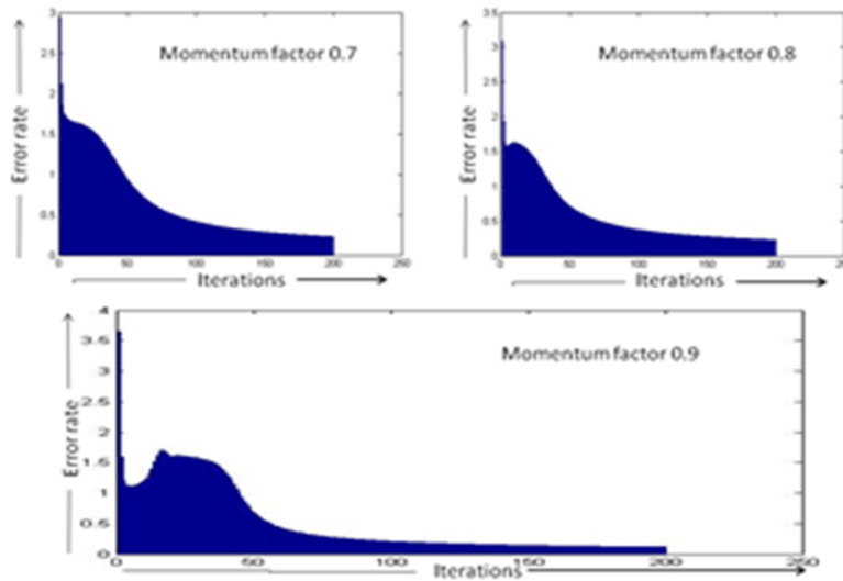
Figure 2 Comparison of various momentum factors
